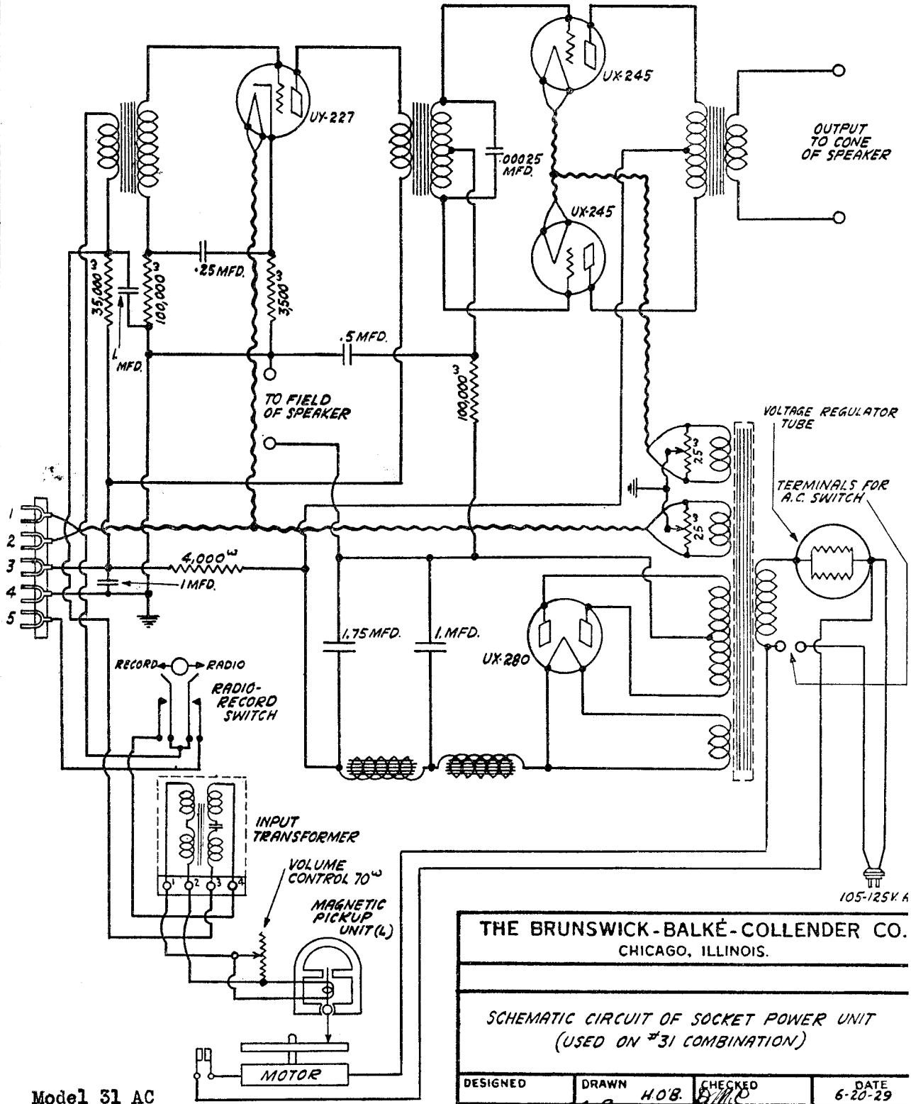
Model 31 AC SPU Schematic
